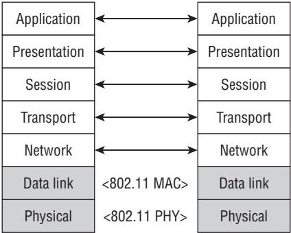
FIGURE 10.1 Wireless LANs in the OSI Model
