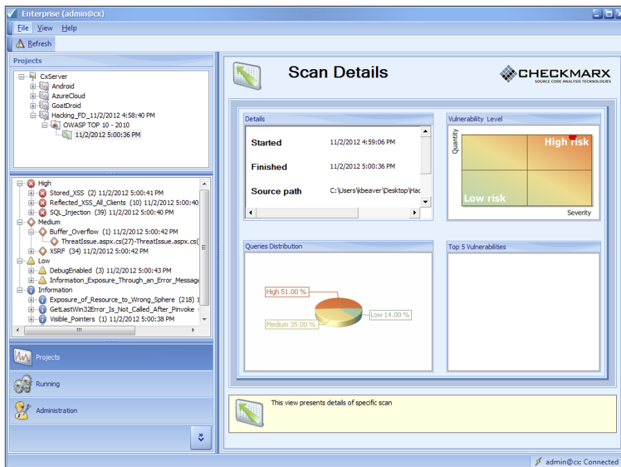
Figure 14-14: Reviewing the results of a CxDeveloper source code analysis.
