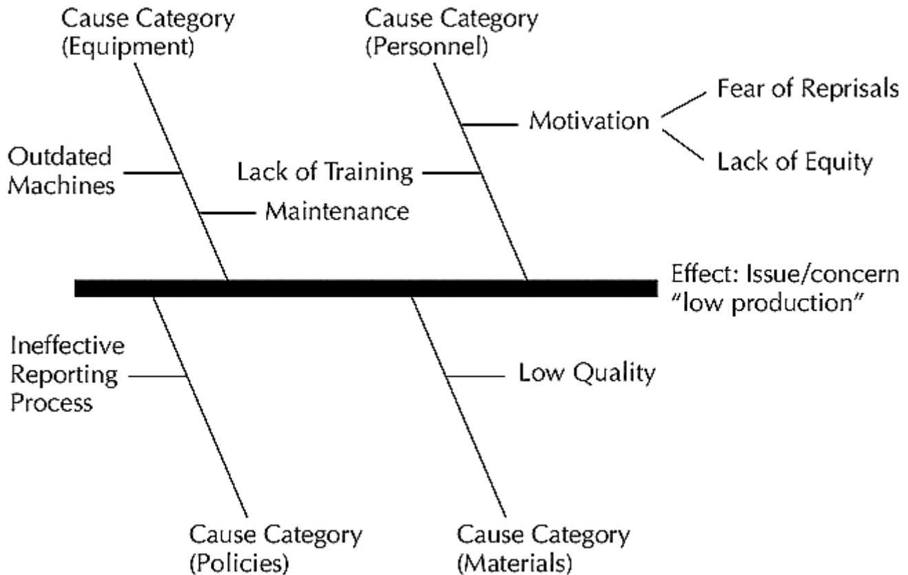
Figure 6.1 Fishbone Diagram
