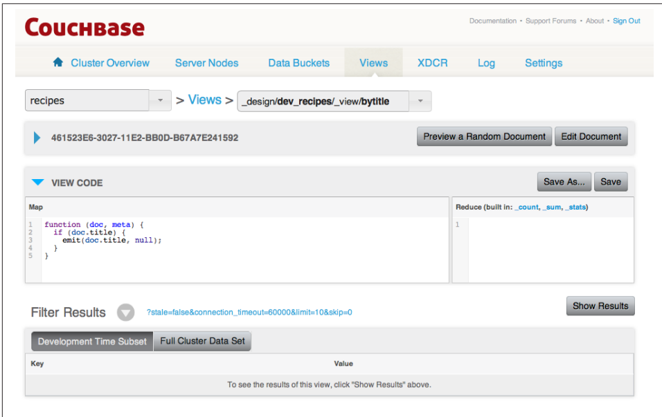
Figure 6-2. Editing Views in the Web Console
