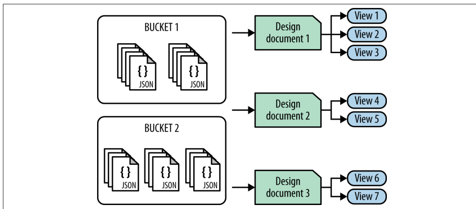
Figure 6-3. Buckets, Design Documents, and Views
