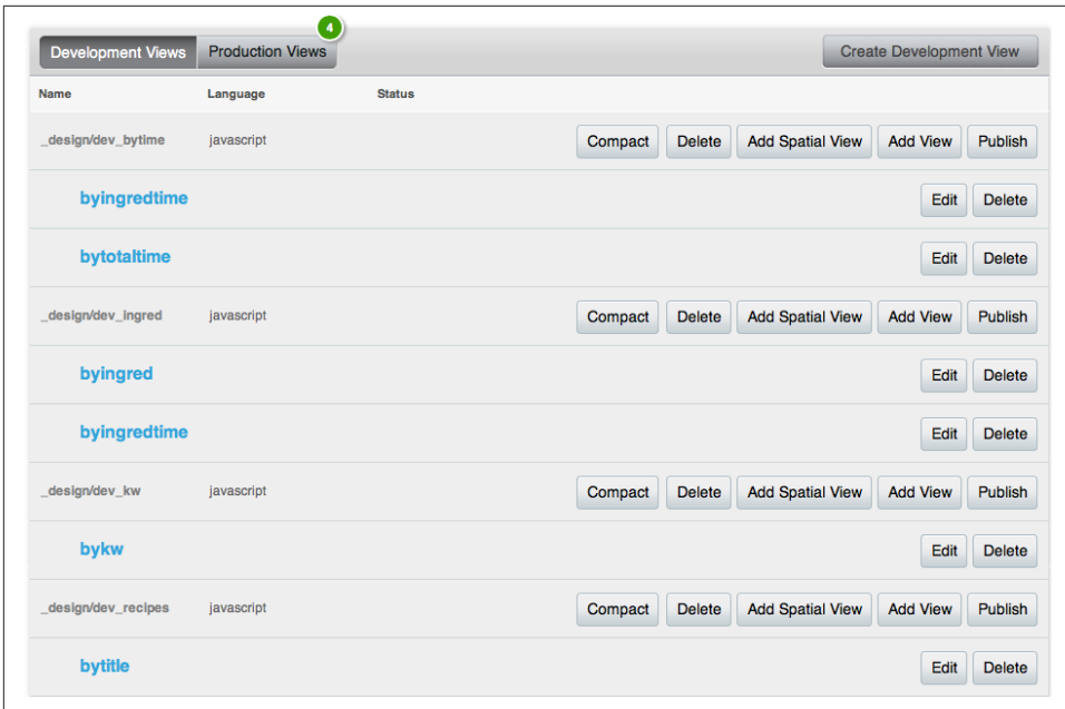
Figure 6-4. Recipe Design Documents and Views
